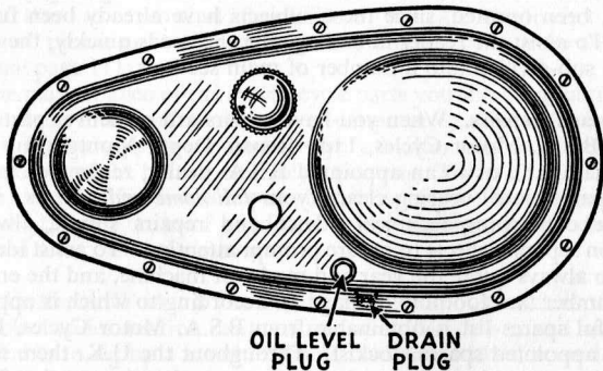
FIG. 37. THE PRESSED-STEEL OIL-BATH CHAIN CASE
