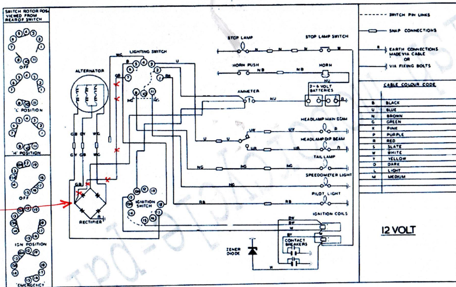
FIG. G.20. Wiring diagram model A65 only.
